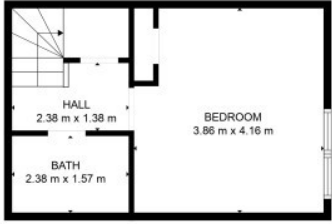
FLOOR 1
