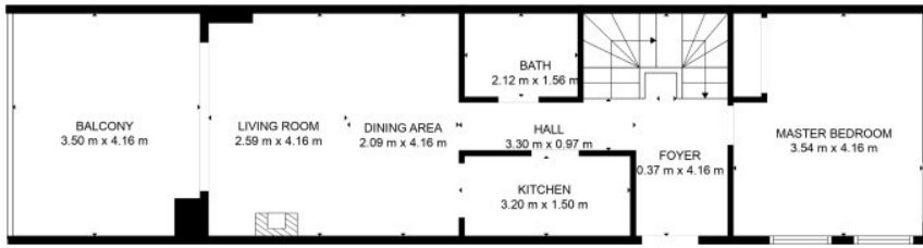
FLOOR 2
