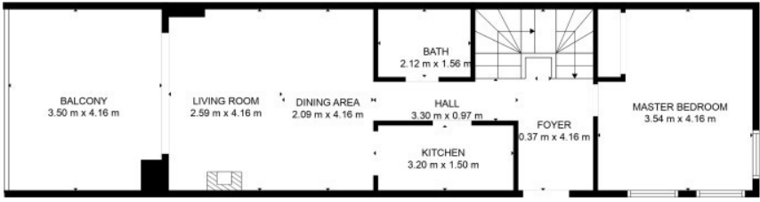
FLOOR 2
