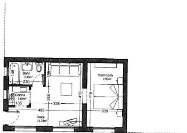
APARTMENT "LOS AMIGOS"
