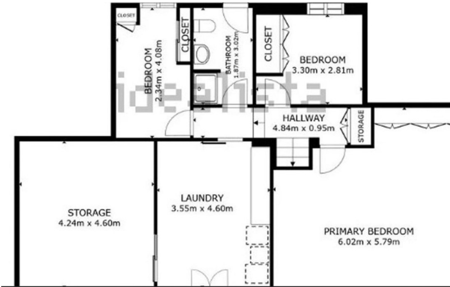
FLOOR 2
