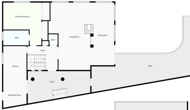
2nd Floor
