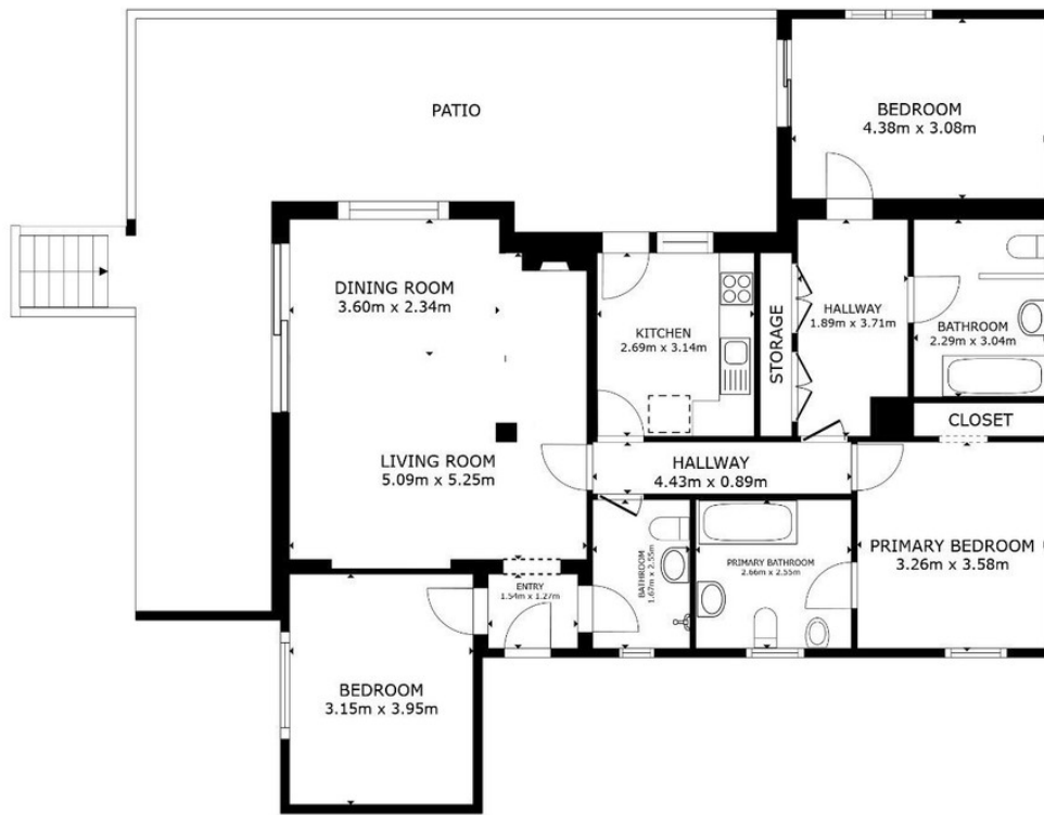
FLOOR PLAN
