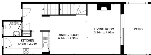
FLOOR 1
